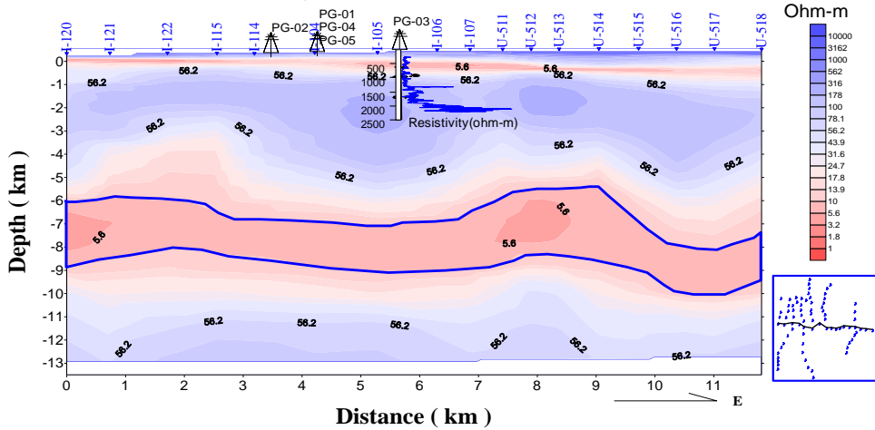
2-D Resistivity Inversion Result of Section 04
