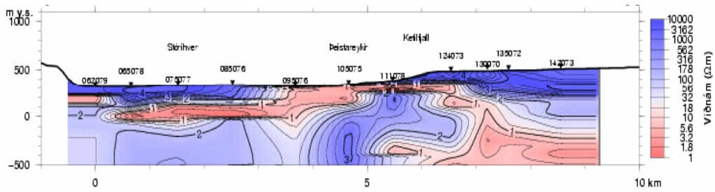
2-D Resistivity Inversion Result of Section 04
